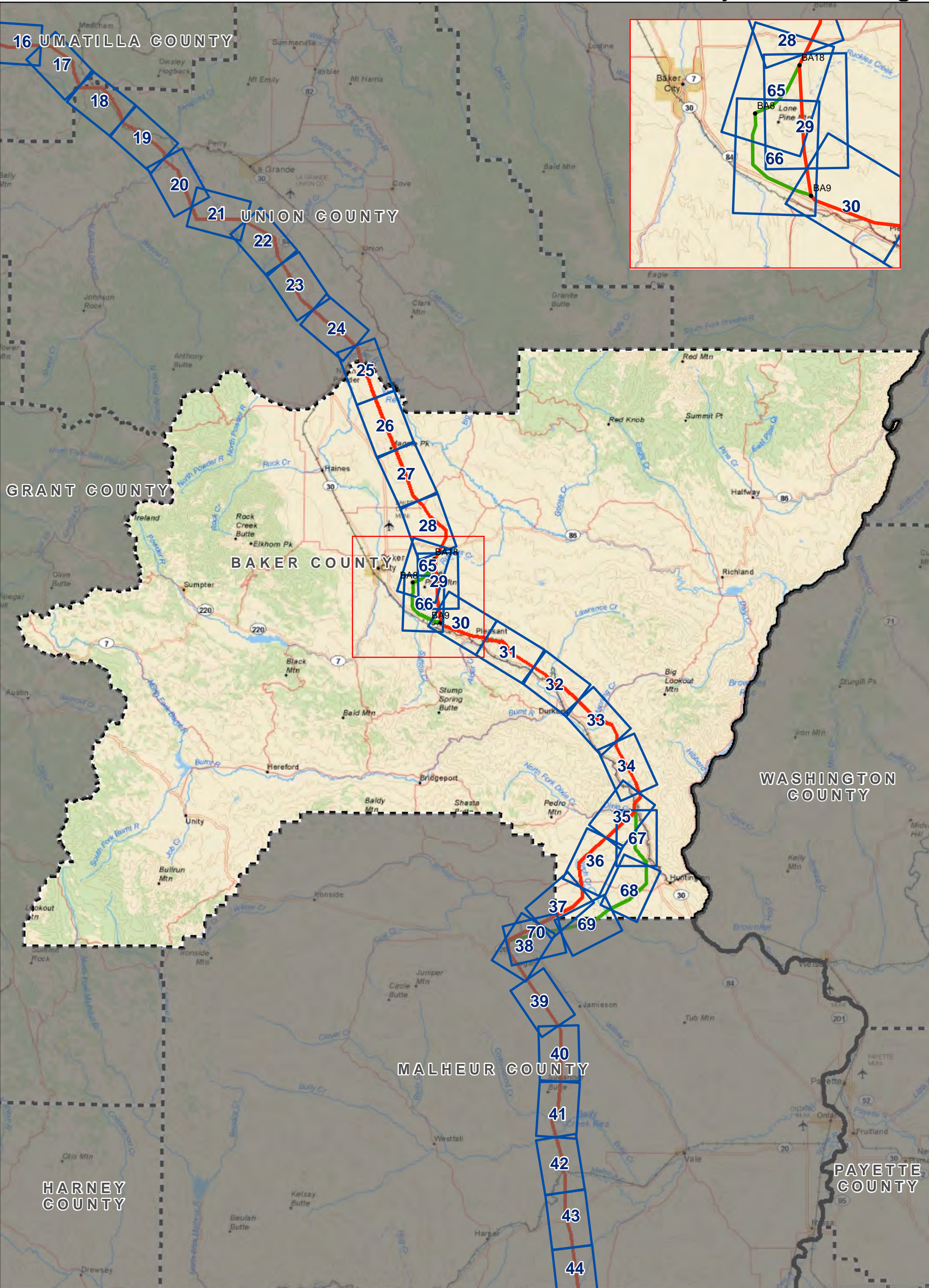
FIGURE 3.1-5 SEGMENT 4 - BAKER COUNTY, OR BOARDMAN TO HEMINGWAY 500kV TRANSMISSION LINE PROJECT OREGON-IDAHO
